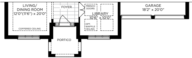
PARTIAL OPT. GROUND FLOOR PLAN ELEV. C
