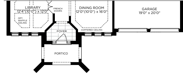
PARTIAL OPT. GROUND FLOOR PLAN ELEV. B
