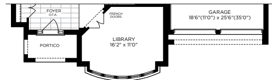
PARTIAL GROUND FLOOR PLAN ELEV. C
