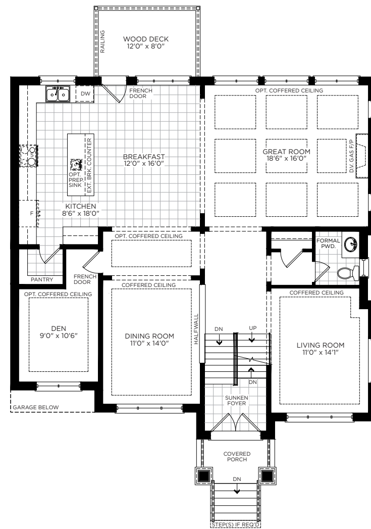
MAIN FLOOR PLAN ELEVATION A, LOT 17
