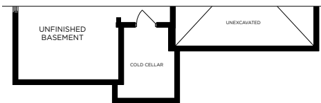
PARTIAL BASEMENT PLAN ELEV. B
