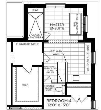
PARTIAL OPT. SECOND FLOOR PLAN MASTER ENSUITE ELEVATION A, B & C
