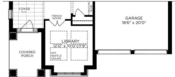
PARTIAL GROUND FLOOR PLAN ELEV. C
