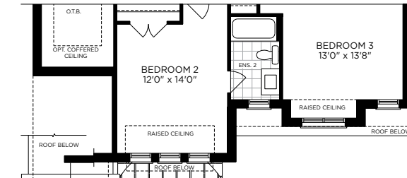
PARTIAL SECOND FLOOR PLAN ELEV. B
