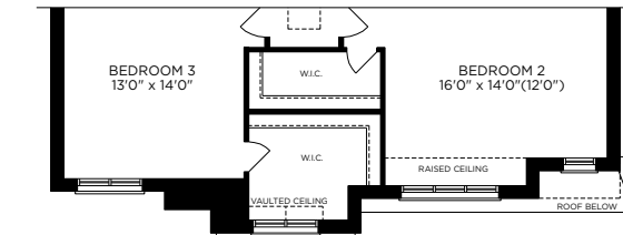
PARTIAL SECOND FLOOR PLAN ELEV. B
