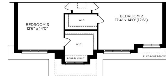
PARTIAL SECOND FLOOR PLAN ELEV. C
