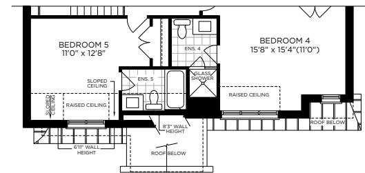
PARTIAL OPT. SECOND FLOOR PLAN ELEV. B
