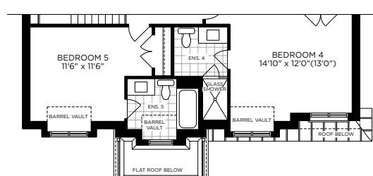
PARTIAL OPT. SECOND FLOOR PLAN ELEV. C
