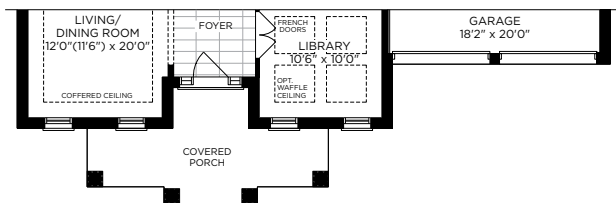
PARTIAL GROUND FLOOR PLAN ELEV. B
