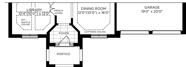
PARTIAL GROUND FLOOR PLAN ELEV. C
