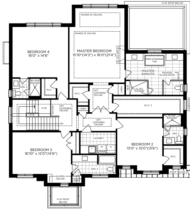
SECOND FLOOR PLAN ELEV. A
