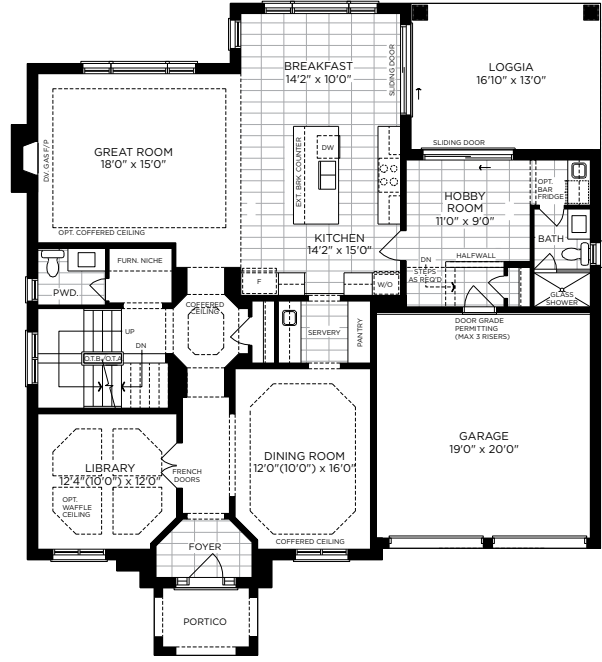
GROUND FLOOR PLAN ELEV. A
