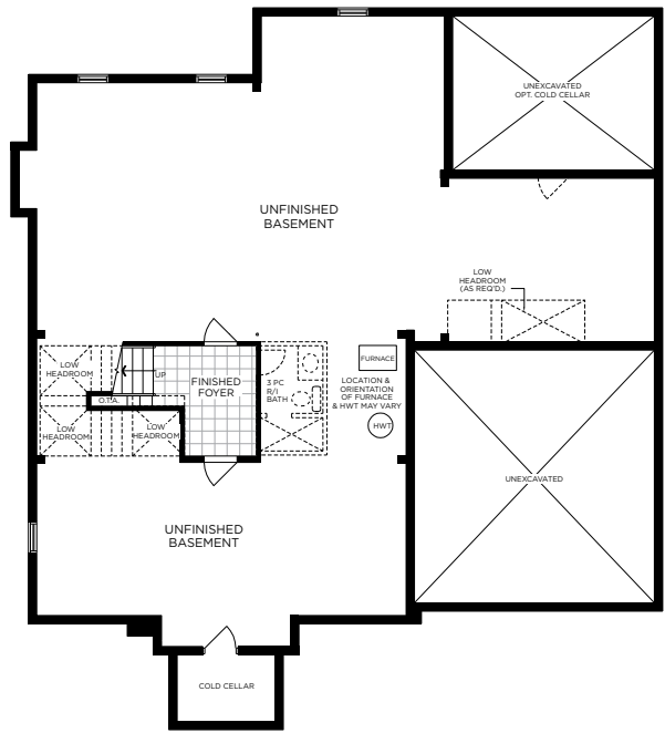
BASEMENT PLAN ELEV. A
