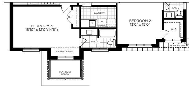
PARTIAL SECOND FLOOR PLAN ELEV. C
