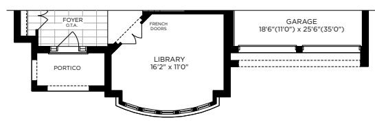
PARTIAL GROUND FLOOR PLAN ELEV. C
