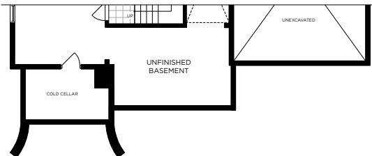
PARTIAL BASEMENT PLAN ELEV. B
