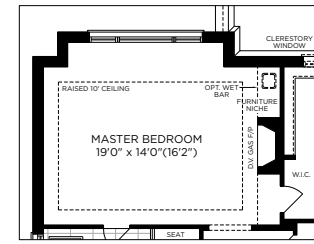
PARTIAL OPTIONAL SECOND FLOOR MASTER BEDROOM W/ WET BAR AND FIREPLACE ELEV. A, B & C
