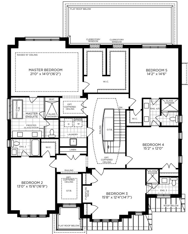
OPTIONAL SECOND FLOOR PLAN ELEV. A
