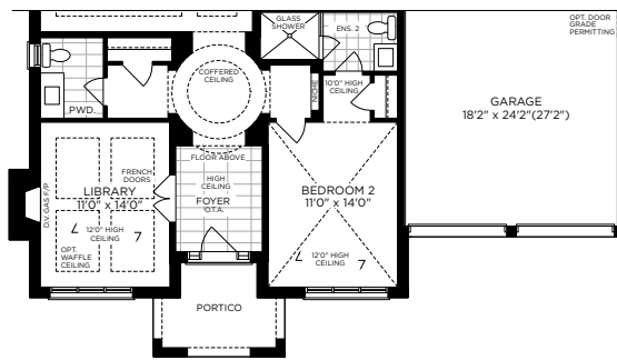
PARTIAL GROUND FLOOR PLAN ELEV. B
