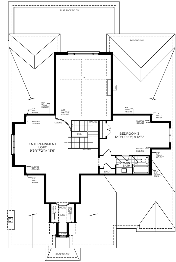
LOFT FLOOR PLAN ELEV. A
