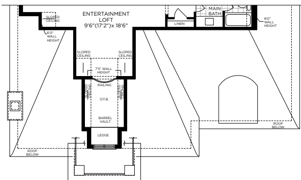
PARTIAL LOFT FLOOR PLAN ELEV. C
