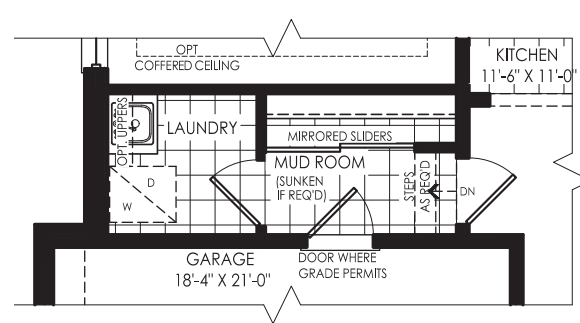
GROUND FLOOR MUD ROOM FOR OPTIONAL SECOND FLOOR ELEVATION A, B AND C
