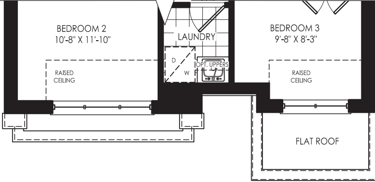
UPPER FLOOR ELEVATION B
