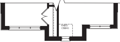
OPTIONAL UPPER FLOOR ELEVATION C
