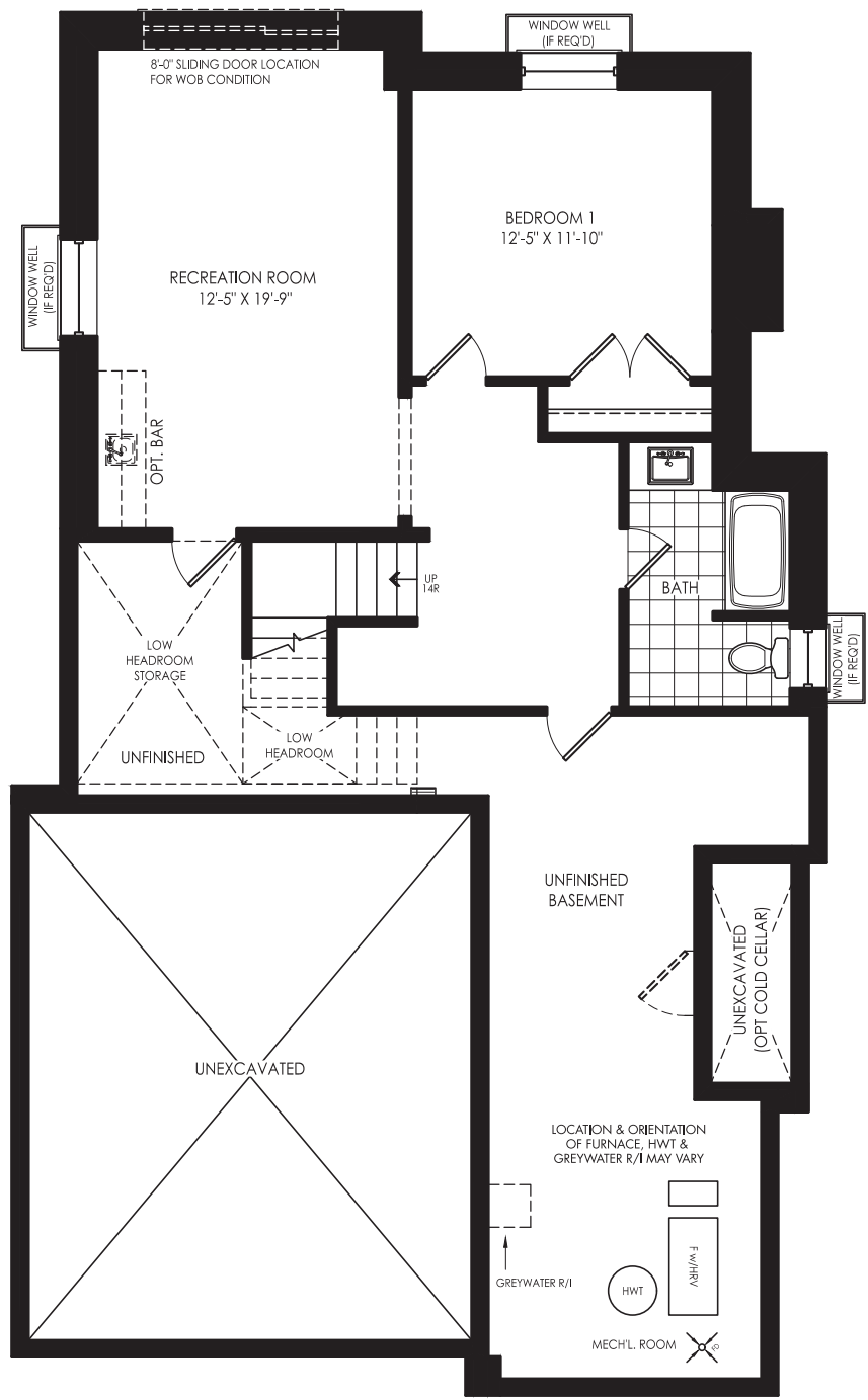
OPTIONAL FINISHED BASEMENT → ELEVATION A 747 - 754 SQ. FT.
