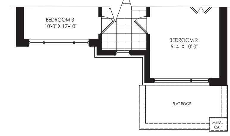
SECOND FLOOR ELEVATION C
