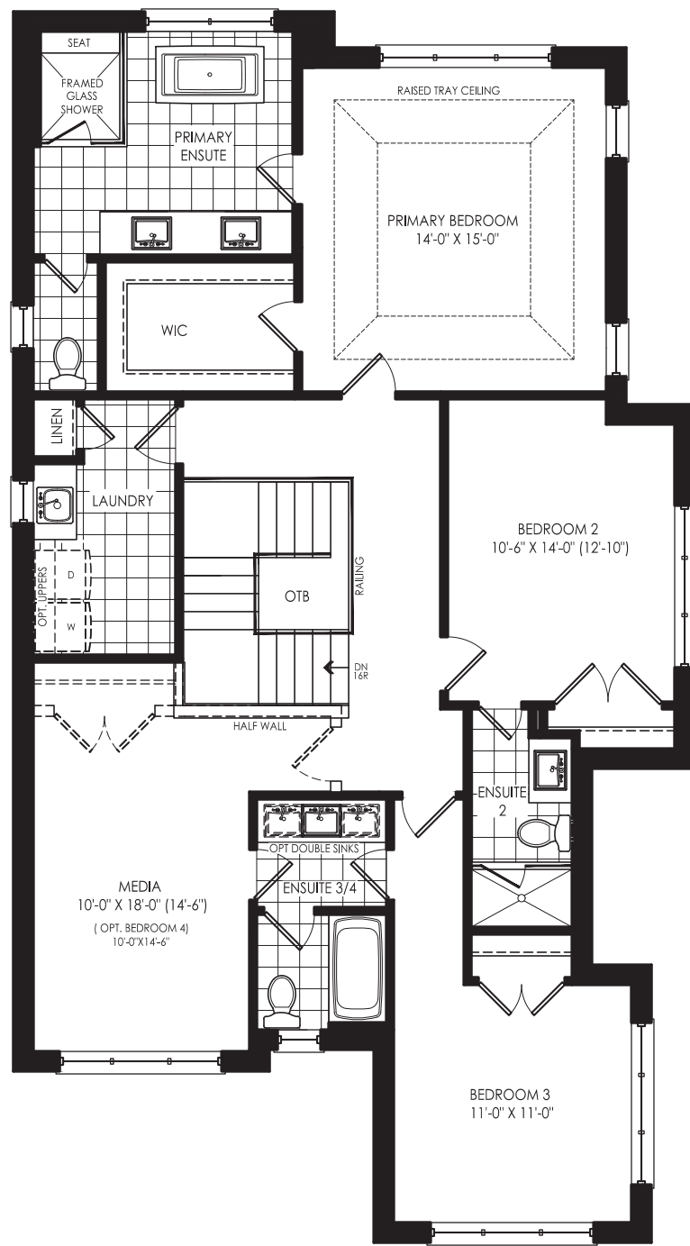
SECOND FLOOR ELEVATION C
