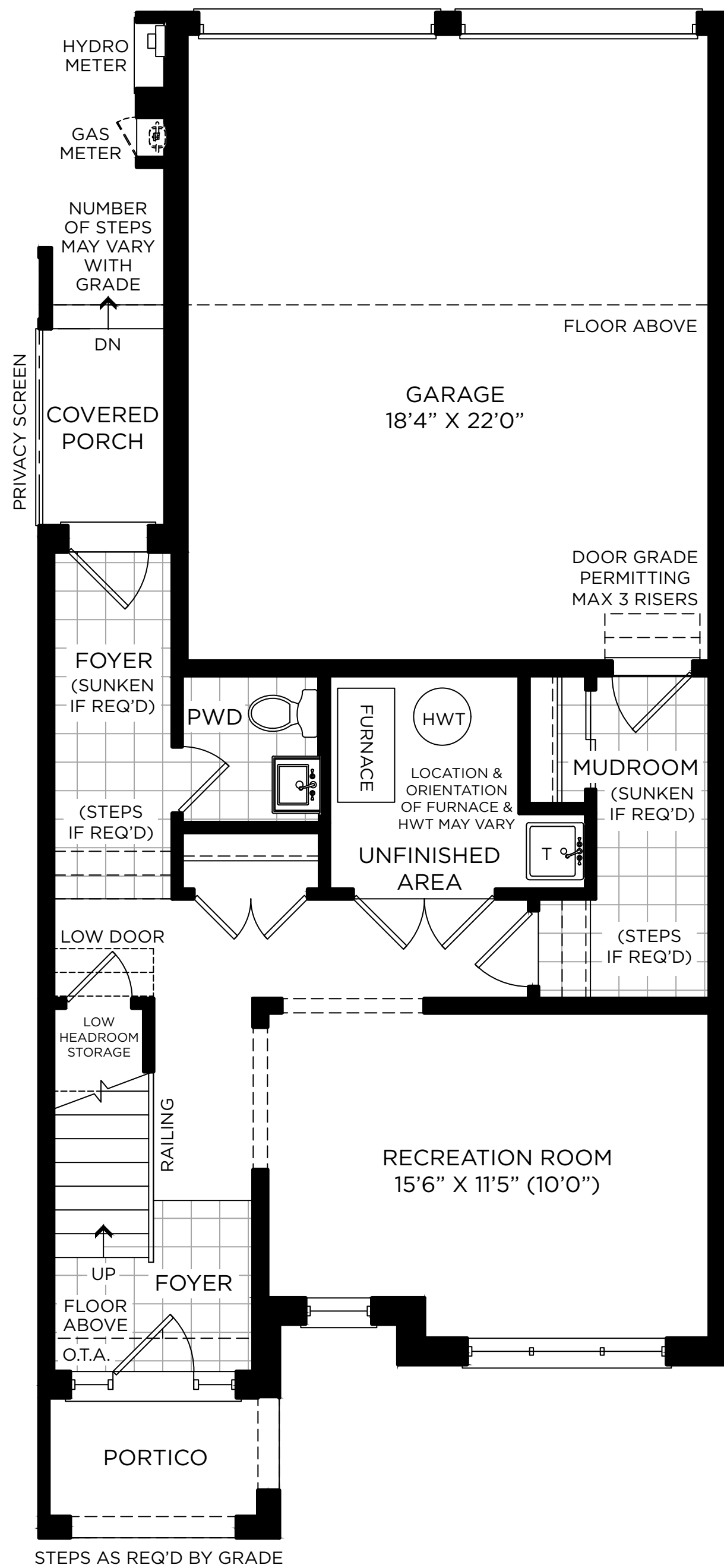
Lower Floor Interior, Block 2, Lots 6 & 9 Elevation B
