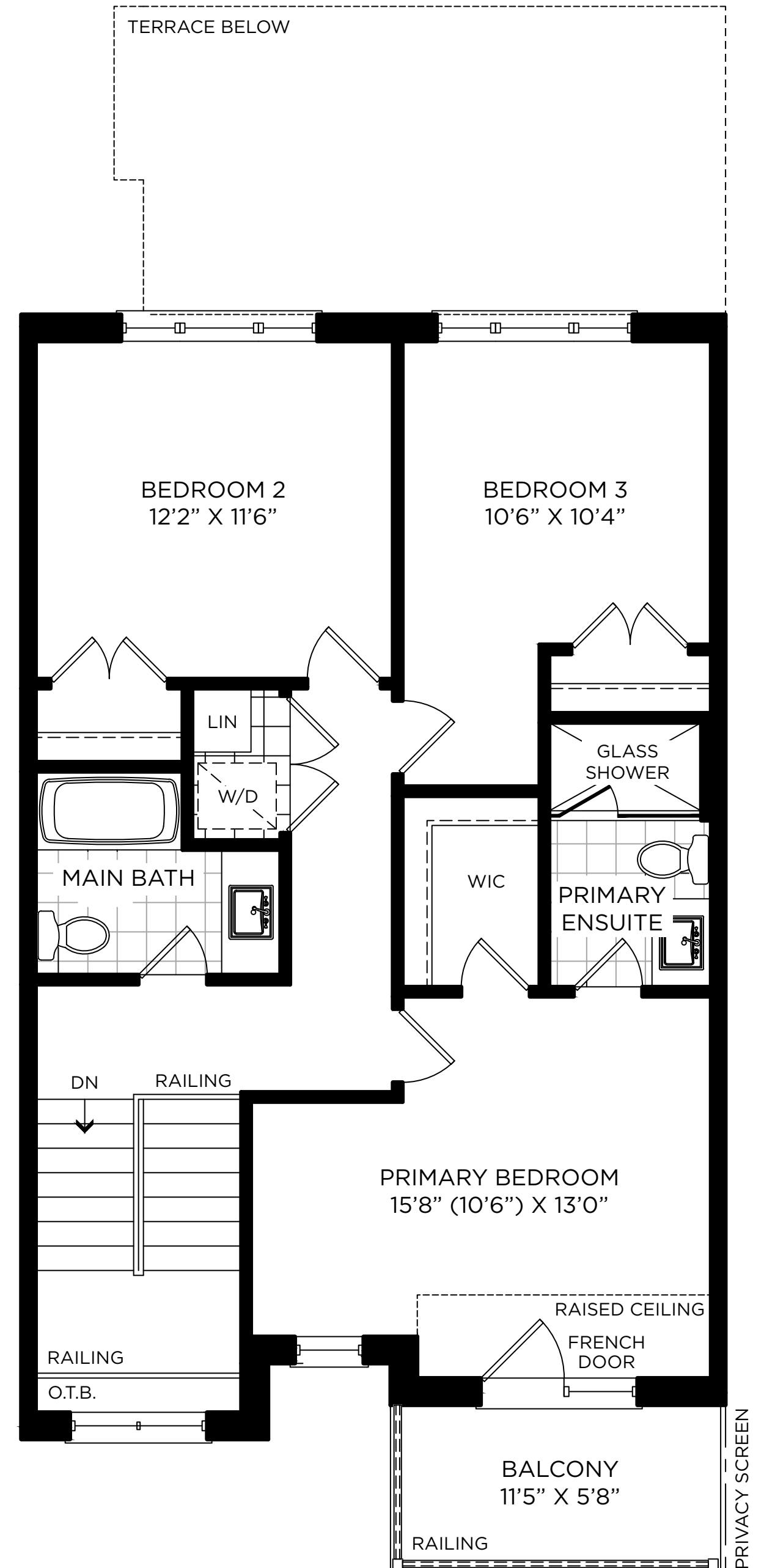
Upper Floor Interior, Block 2, Lots 6 & 9 Elevation B
