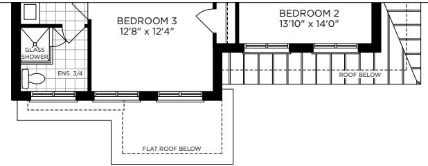
PARTIAL SECOND FLOOR PLAN ELEV. C
