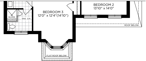
PARTIAL SECOND FLOOR PLAN ELEV. B
