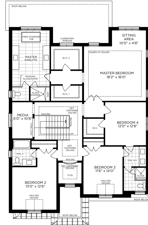
OPTIONAL SECOND FLOOR PLAN ELEV. A
