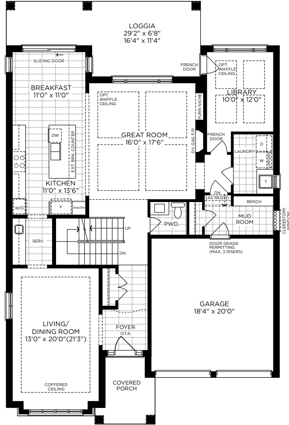
GROUND FLOOR PLAN ELEV. A
