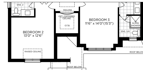
PARTIAL OPT. SECOND FLOOR PLAN ELEV. B
