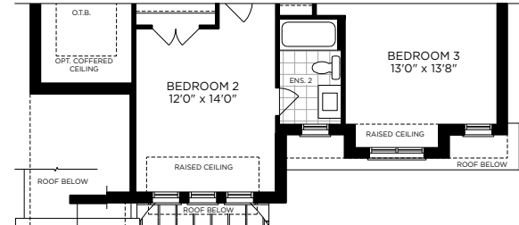
PARTIAL SECOND FLOOR PLAN ELEV. B
