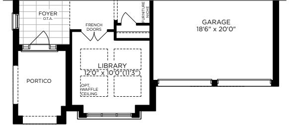
PARTIAL GROUND FLOOR PLAN ELEV. B
