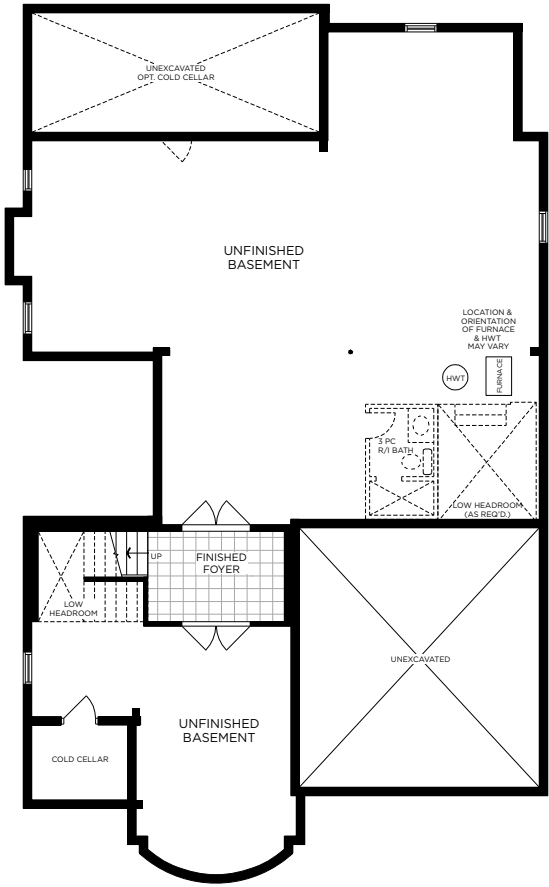
BASEMENT PLAN ELEV. A
