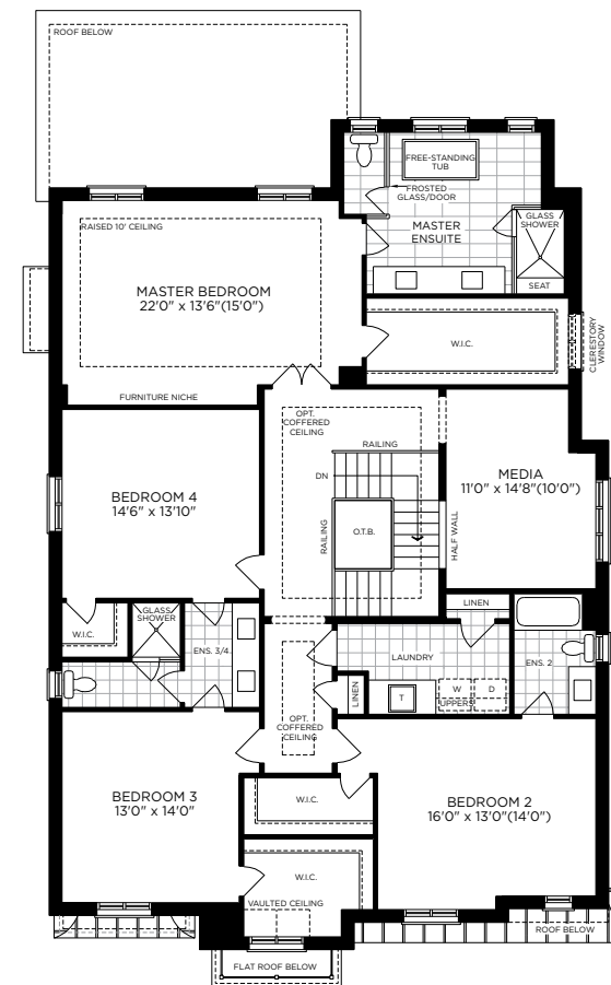
SECOND FLOOR PLAN ELEV. A
