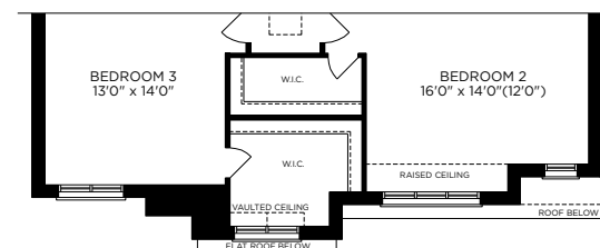
PARTIAL SECOND FLOOR PLAN ELEV. B
