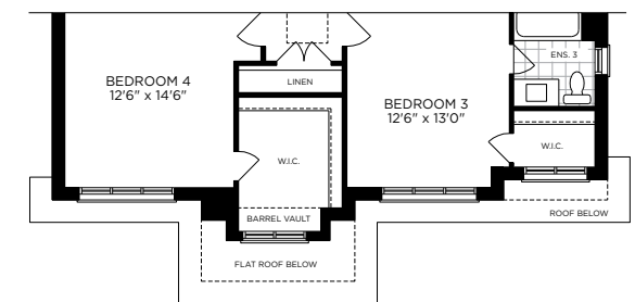
PARTIAL OPT. SECOND FLOOR PLAN ELEV. C
