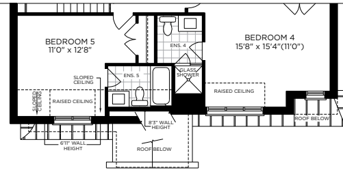
PARTIAL OPT. SECOND FLOOR PLAN ELEV. B
