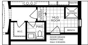
PARTIAL GROUND FLOOR PLAN W/ OPT. DOG SHOWER ELEVATIONS A, B, & C
