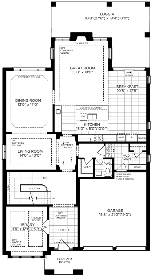
GROUND FLOOR PLAN ELEV. A
