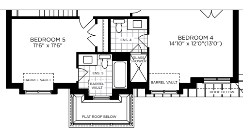
PARTIAL OPT. SECOND FLOOR PLAN ELEV. C
