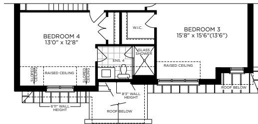
PARTIAL SECOND FLOOR PLAN ELEV. B
