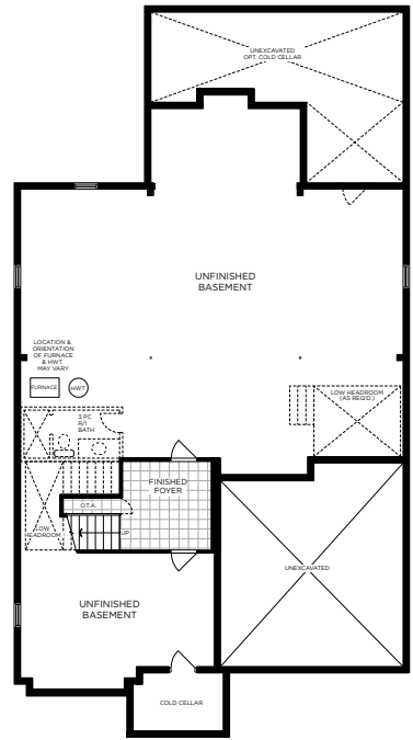
BASEMENT PLAN ELEV. A
