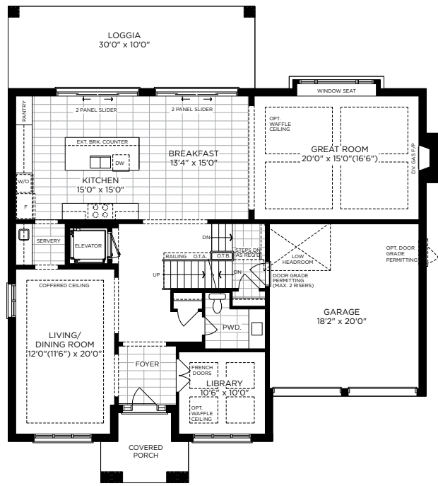
OPTIONAL GROUND FLOOR PLAN ELEV. A
