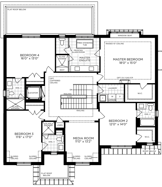
OPTIONAL SECOND FLOOR PLAN ELEV. A
