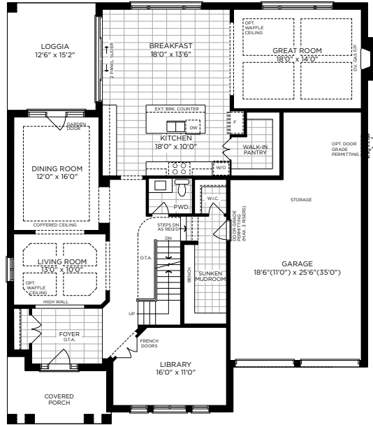
GROUND FLOOR PLAN ELEV. A
