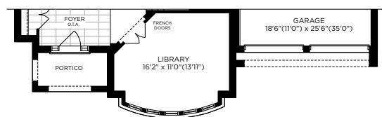
PARTIAL GROUND FLOOR PLAN ELEV. C
