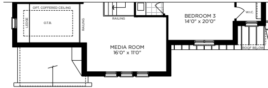
PARTIAL SECOND FLOOR PLAN ELEV. B
