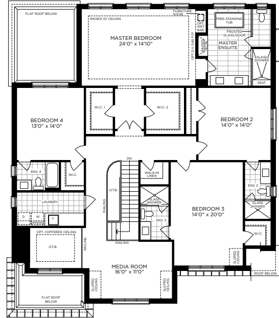
SECOND FLOOR PLAN ELEV. A
