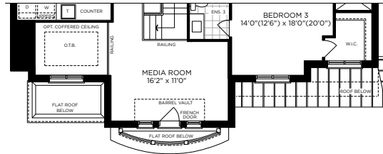
PARTIAL SECOND FLOOR PLAN ELEV. C
