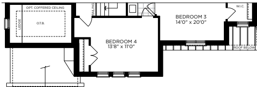
PARTIAL OPT. SECOND FLOOR PLAN ELEV. B
