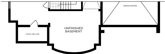
PARTIAL BASEMENT PLAN ELEV. C
