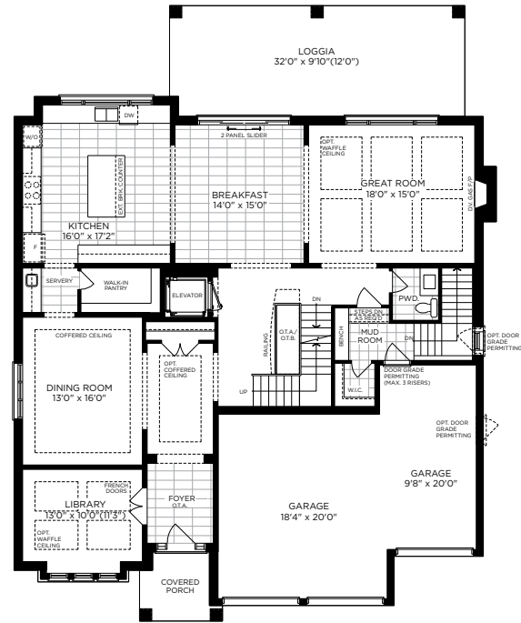
OPTIONAL GROUND FLOOR PLAN ELEV. A
