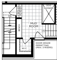
PARTIAL OPTIONAL GROUND FLOOR PLAN WITH DOG SHOWER ELEV. A, B & C
