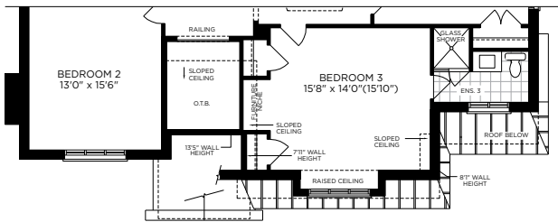
PARTIAL OPT. SECOND FLOOR PLAN ELEV. B
