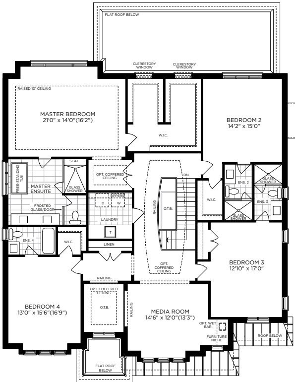
SECOND FLOOR PLAN ELEV. A
