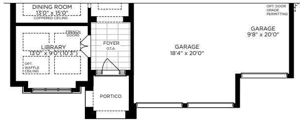
PARTIAL GROUND FLOOR PLAN ELEV. C
