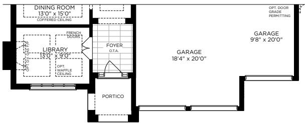
PARTIAL GROUND FLOOR PLAN ELEV. B
