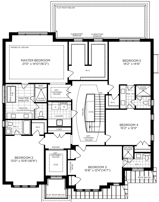
OPTIONAL SECOND FLOOR PLAN ELEV. A
