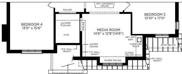
PARTIAL SECOND FLOOR PLAN ELEV. B
