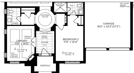
PARTIAL GROUND FLOOR PLAN ELEV. B
