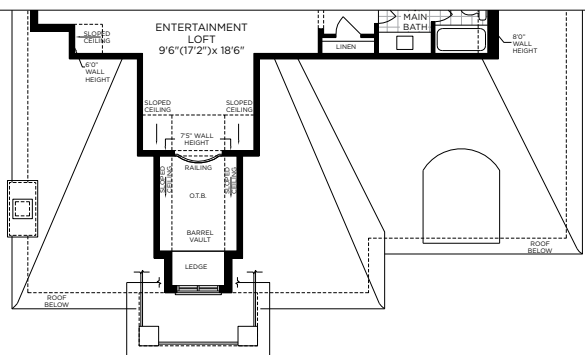
PARTIAL LOFT FLOOR PLAN ELEV. C
