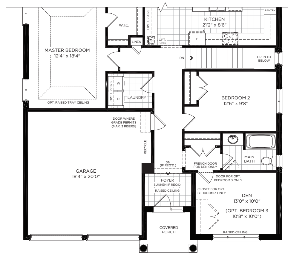
OPT. GROUND FLOOR DEN, ELEVATION C
