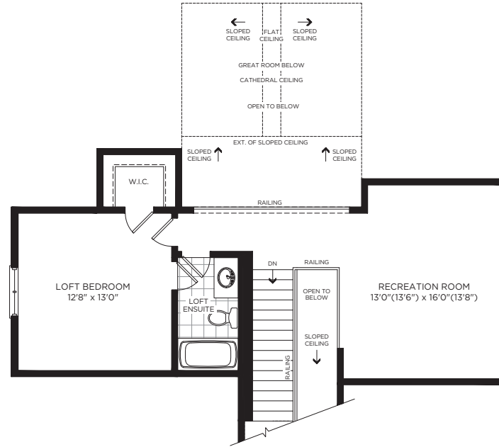
OPT. LOFT, ELEVATION A
