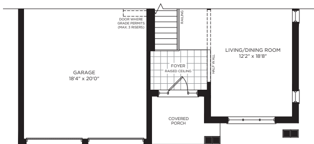
GROUND FLOOR, ELEVATION B (SAME FOR OPT. LOFT GROUND FLOOR, ELEVATION B & OPT. GROUND FLOOR 3 BEDROOM, ELEVATION B)
