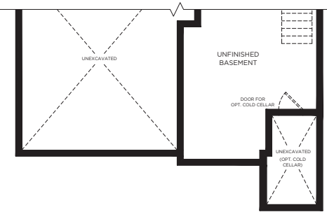
BASEMENT ELEVATION B
