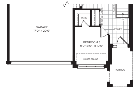
OPT. GROUND FLOOR, 3 BEDROOM, ELEVATION B
