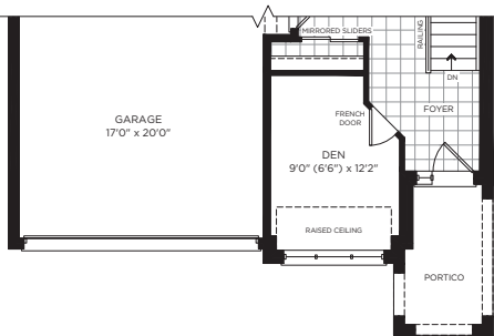
GROUND FLOOR, ELEVATION B
