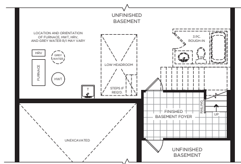
OPT. BASEMENT LOFT, ELEVATION A & B
