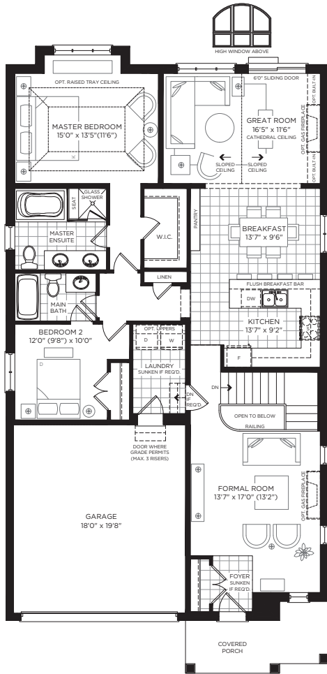
GROUND FLOOR, ELEVATION A
