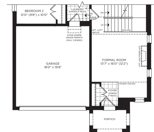
OPT. GROUND FLOOR LOFT, ELEVATION B
