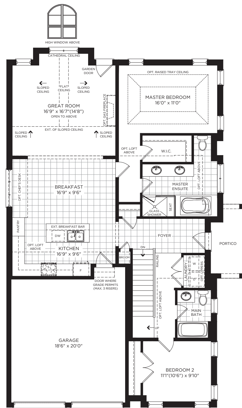
OPT. GROUND FLOOR LOFT, ELEVATION B
