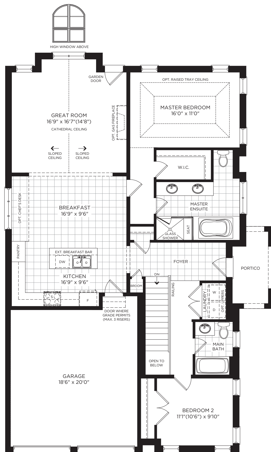
GROUND FLOOR, ELEVATION B
