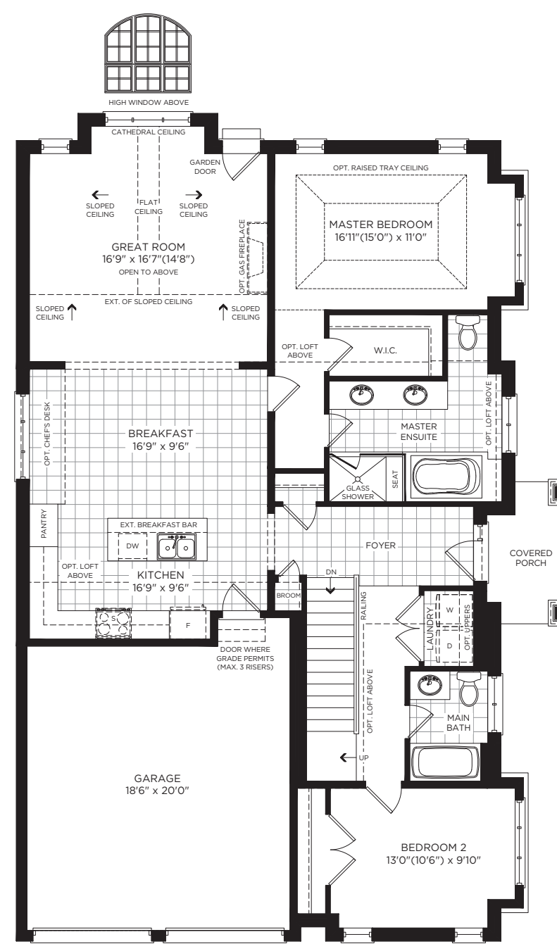
OPT. GROUND FLOOR LOFT, ELEVATION A
