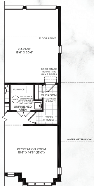
Lower Floor Interior End, Block 3, Lot 11 Elevation A, Total 2,585 sq. ft.
