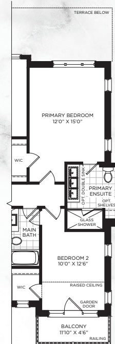
Partial Upper Floor Exterior End, Block 3, Lot 14 Elevation A
