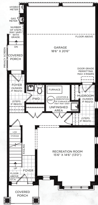
Lower Floor Interior End, Block 3, Lot 11 Elevation A, Total 2,585 sq. ft.
