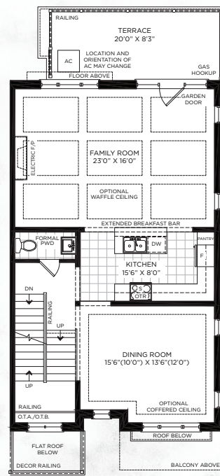
Main Floor Interior End, Block 3, Lot 11 Elevation A
