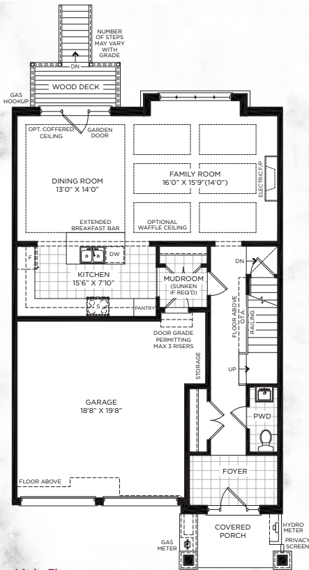
Main Floor Interior, Block 5, Lots 20 & 21 Elevation A
