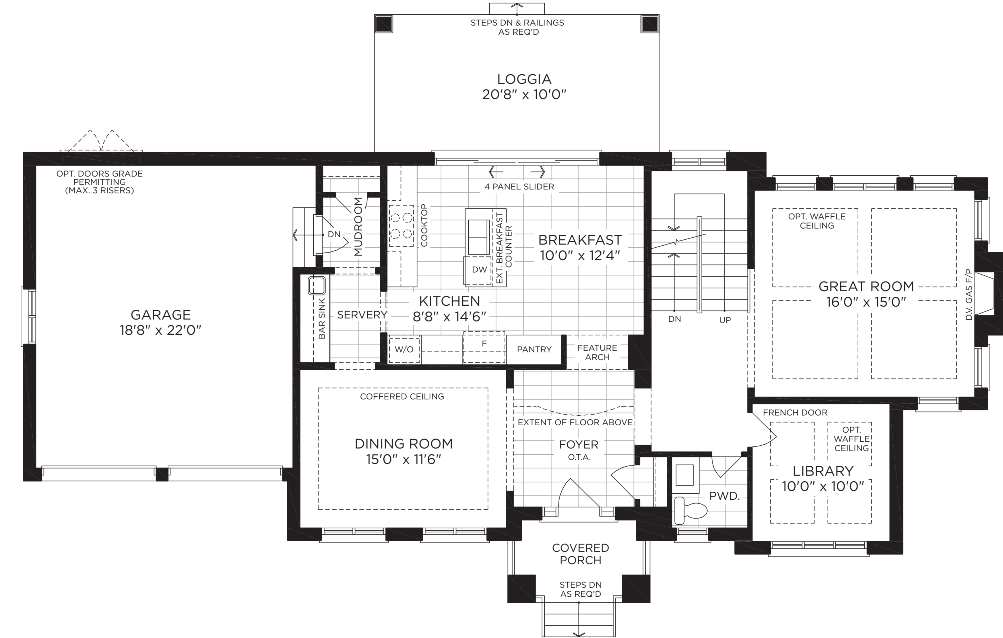
GROUND FLOOR PLAN ELEV. C
