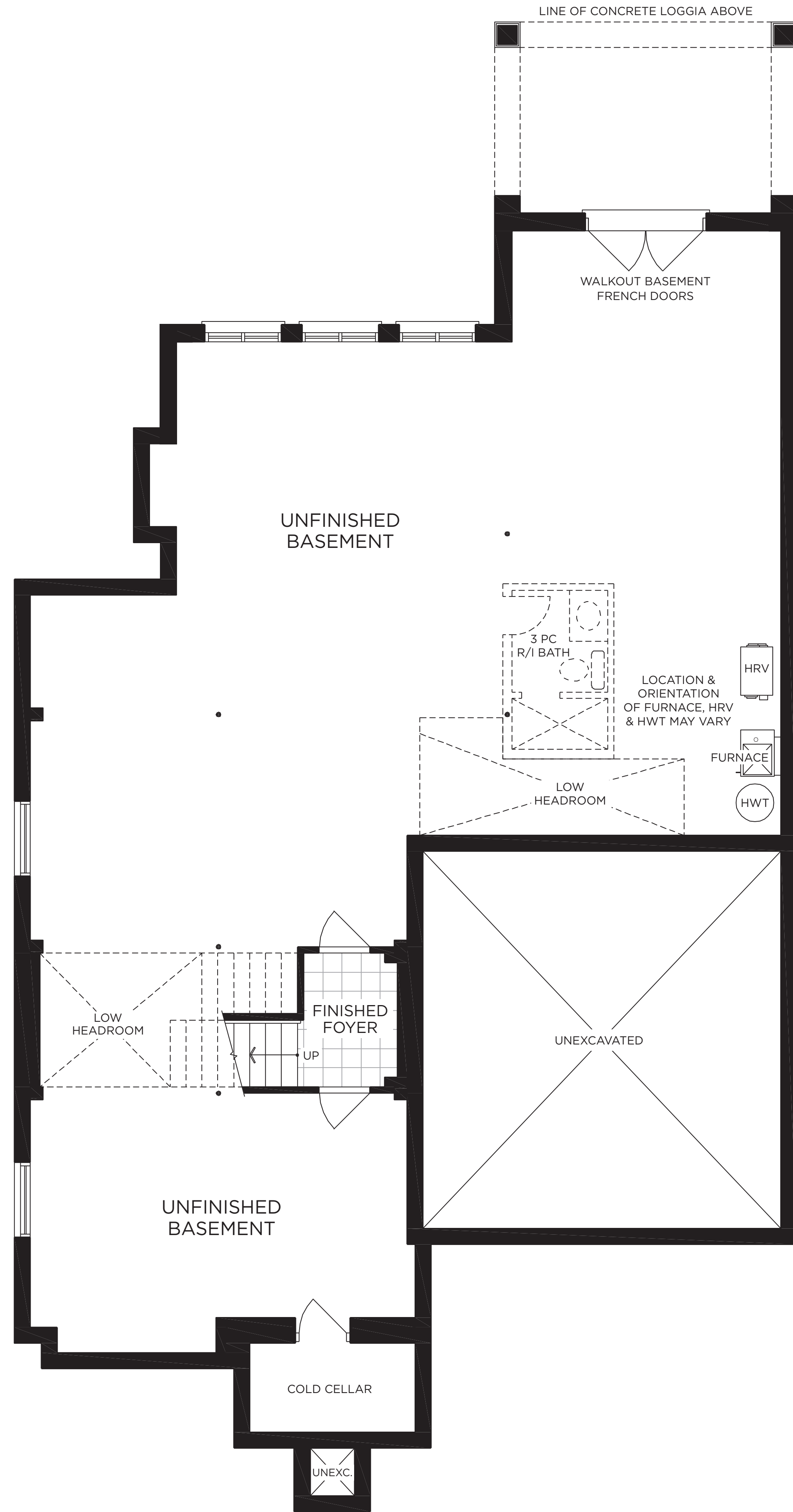
BASEMENT PLAN ELEV. C
