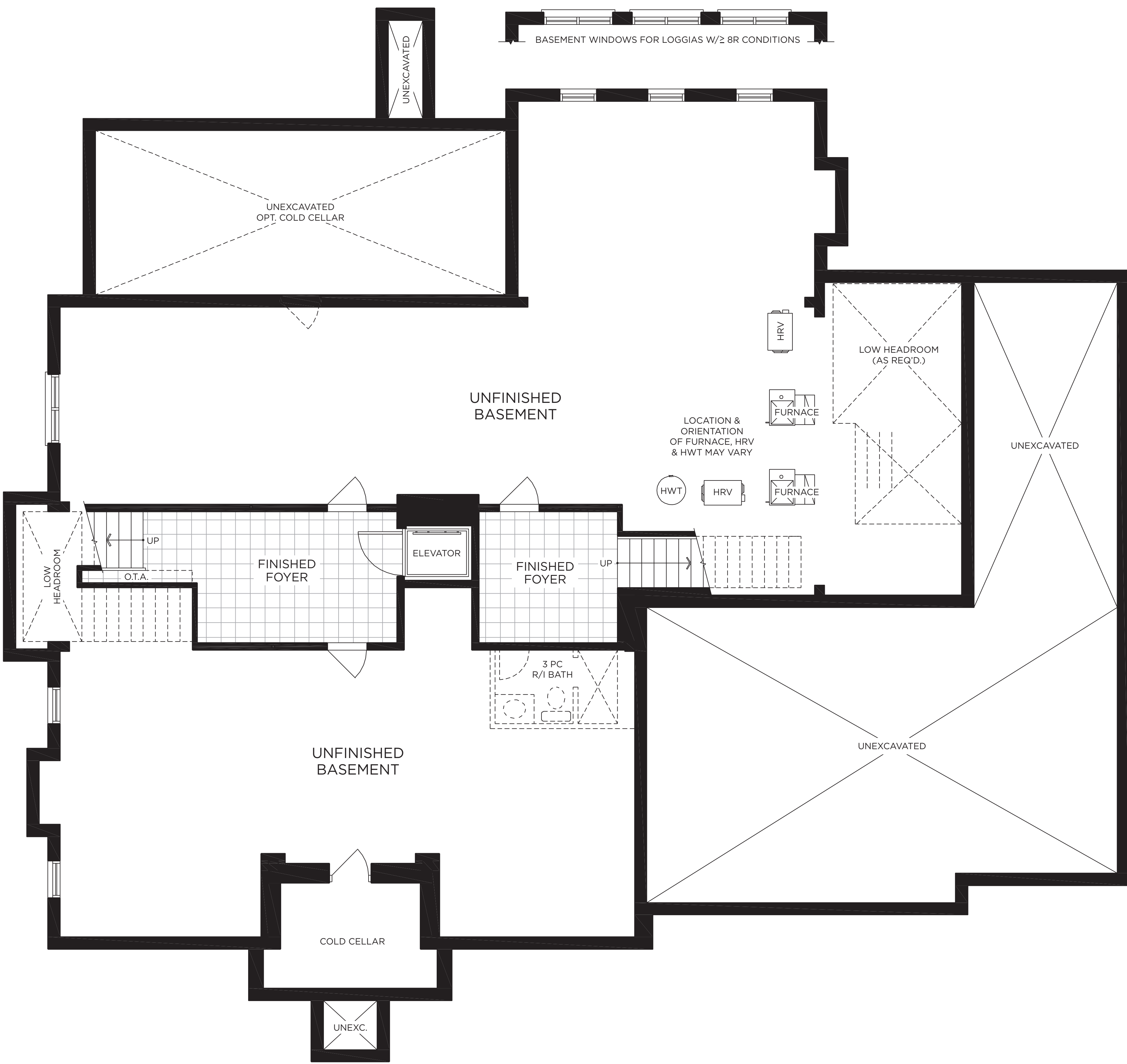
OPT. BASEMENT PLAN W/ELEVATOR, ELEV. C
