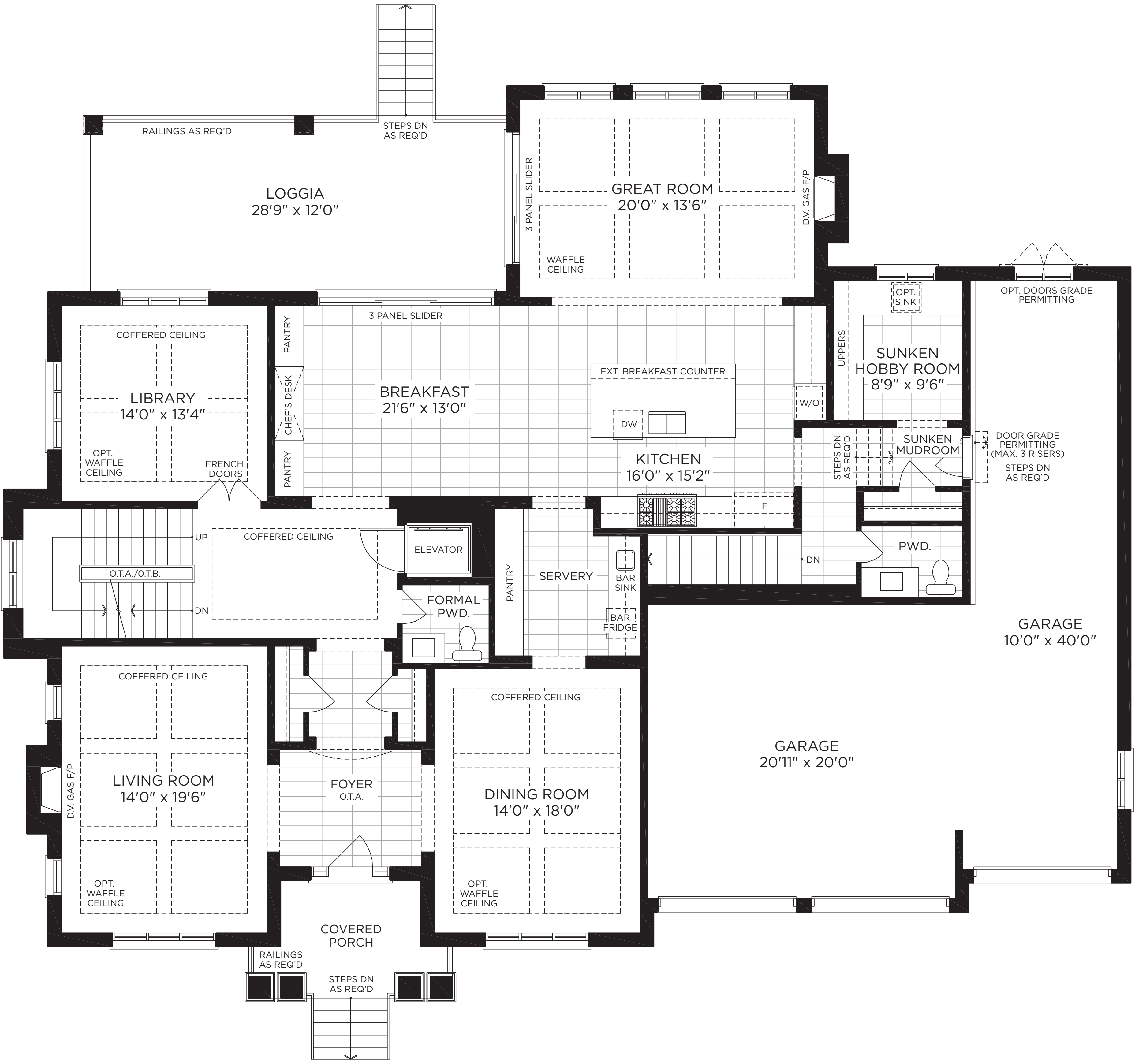
OPT. GROUND FLOOR PLAN W/ELEVATOR, ELEV. C
