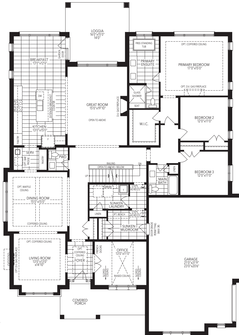
GROUND FLOOR W/OPT. LOFT ELEVATION B
