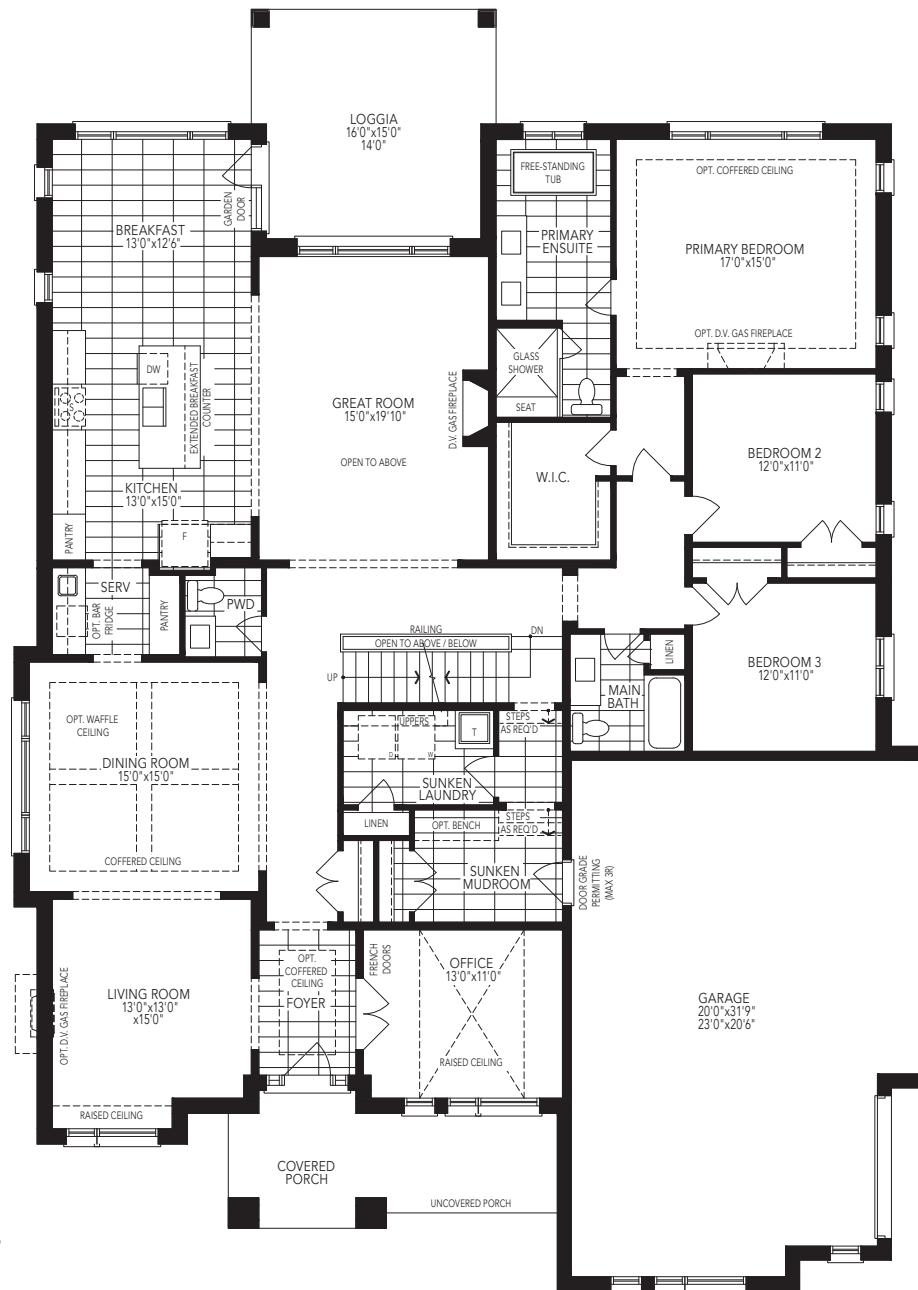
GROUND FLOOR W/OPT. LOFT ELEVATION C
