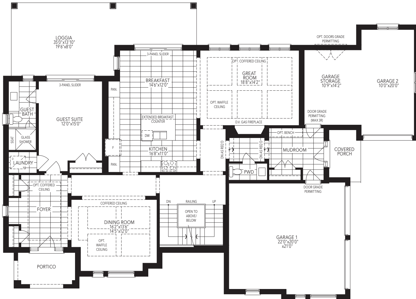
GROUND FLOOR W/OPT. GUEST SUITE ELEVATION C
