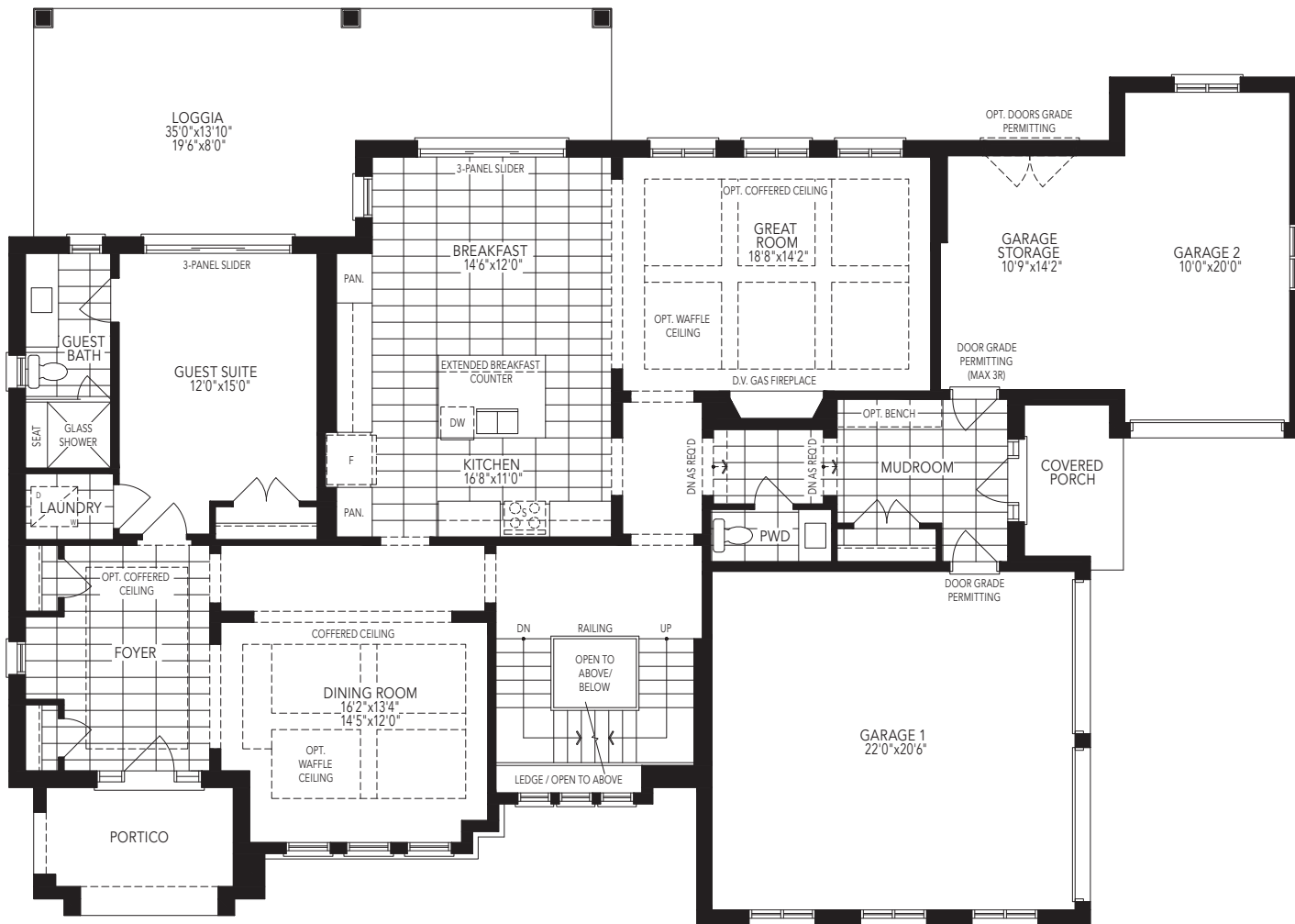
GROUND FLOOR W/OPT. GUEST SUITE ELEVATION B
