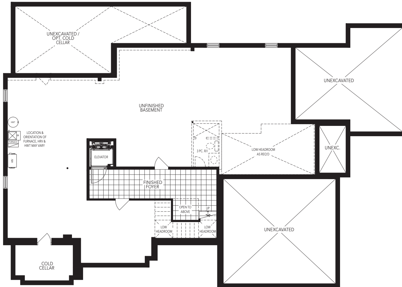
BASEMENT W/OPT. ELEVATOR + GUEST SUITE ELEVATION B
