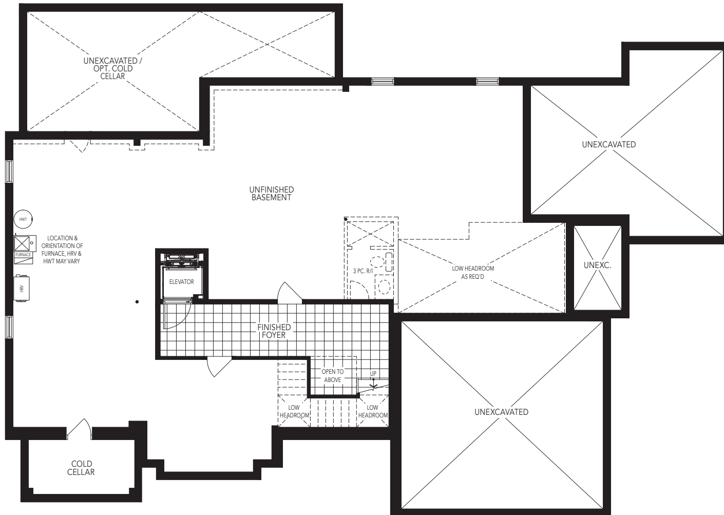
BASEMENT W/OPT. ELEVATOR ELEVATION A
