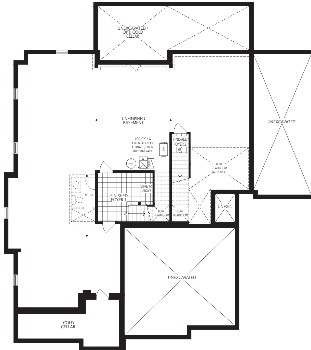
BASEMENT W/OPT. SERVICE STAIRS ELEVATION C
