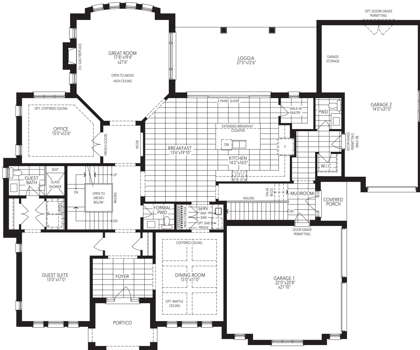
GROUND FLOOR W/OPT. GUEST SUITE ELEVATION A
