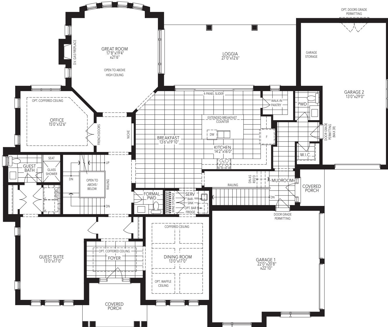
GROUND FLOOR W/OPT. GUEST SUITE ELEVATION C
