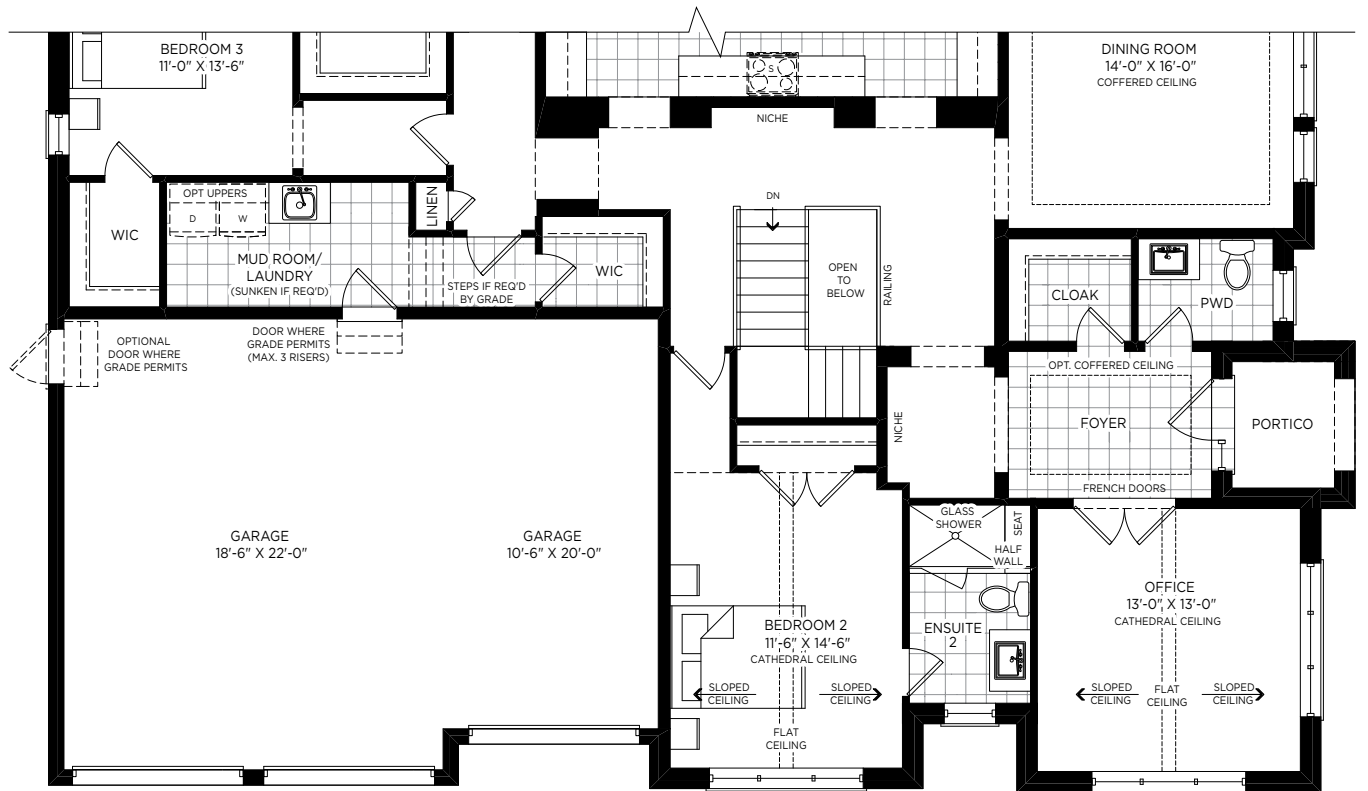
GROUND FLOOR ELEVATION B
