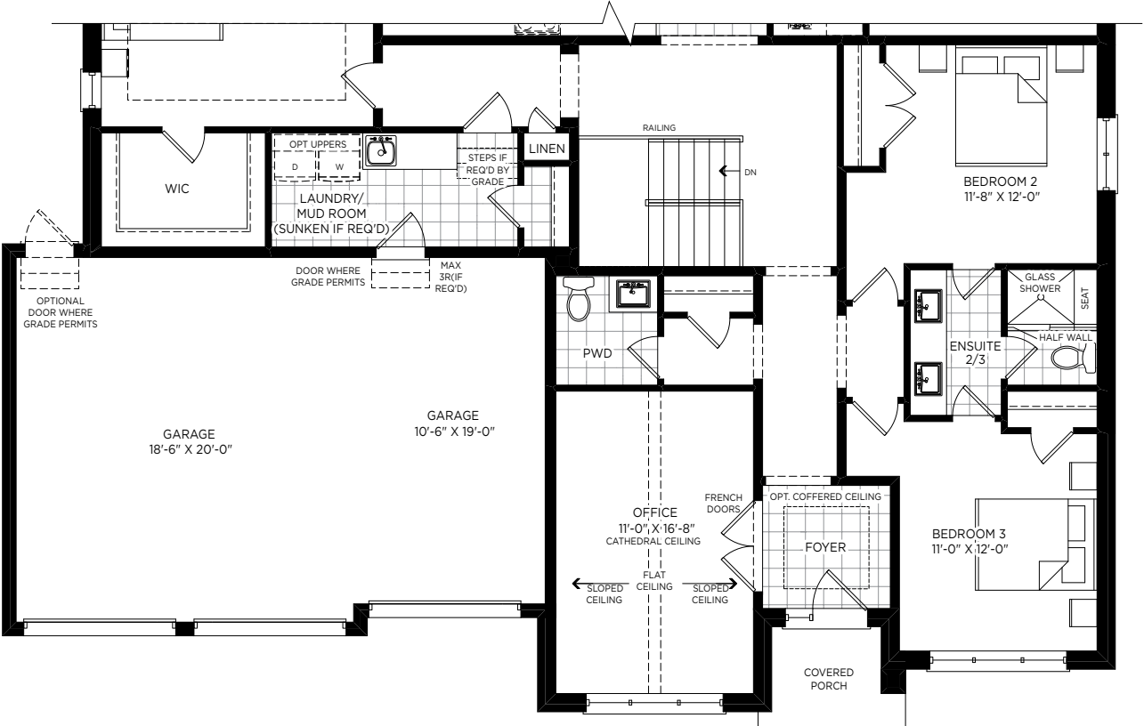
OPT. GROUND FLOOR WITH THIRD BEDROOM ELEVATION B
