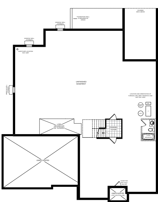
BASEMENT ELEVATION B
