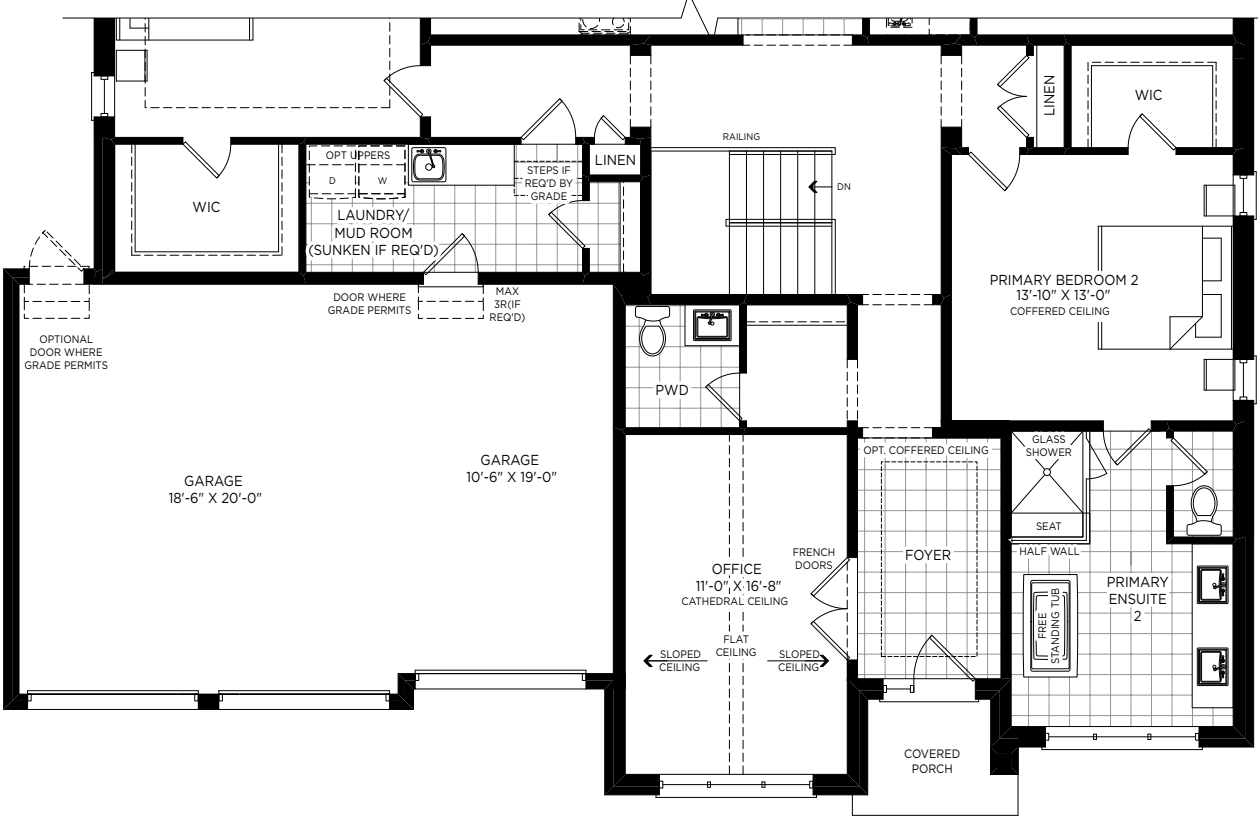
GROUND FLOOR ELEVATION B
