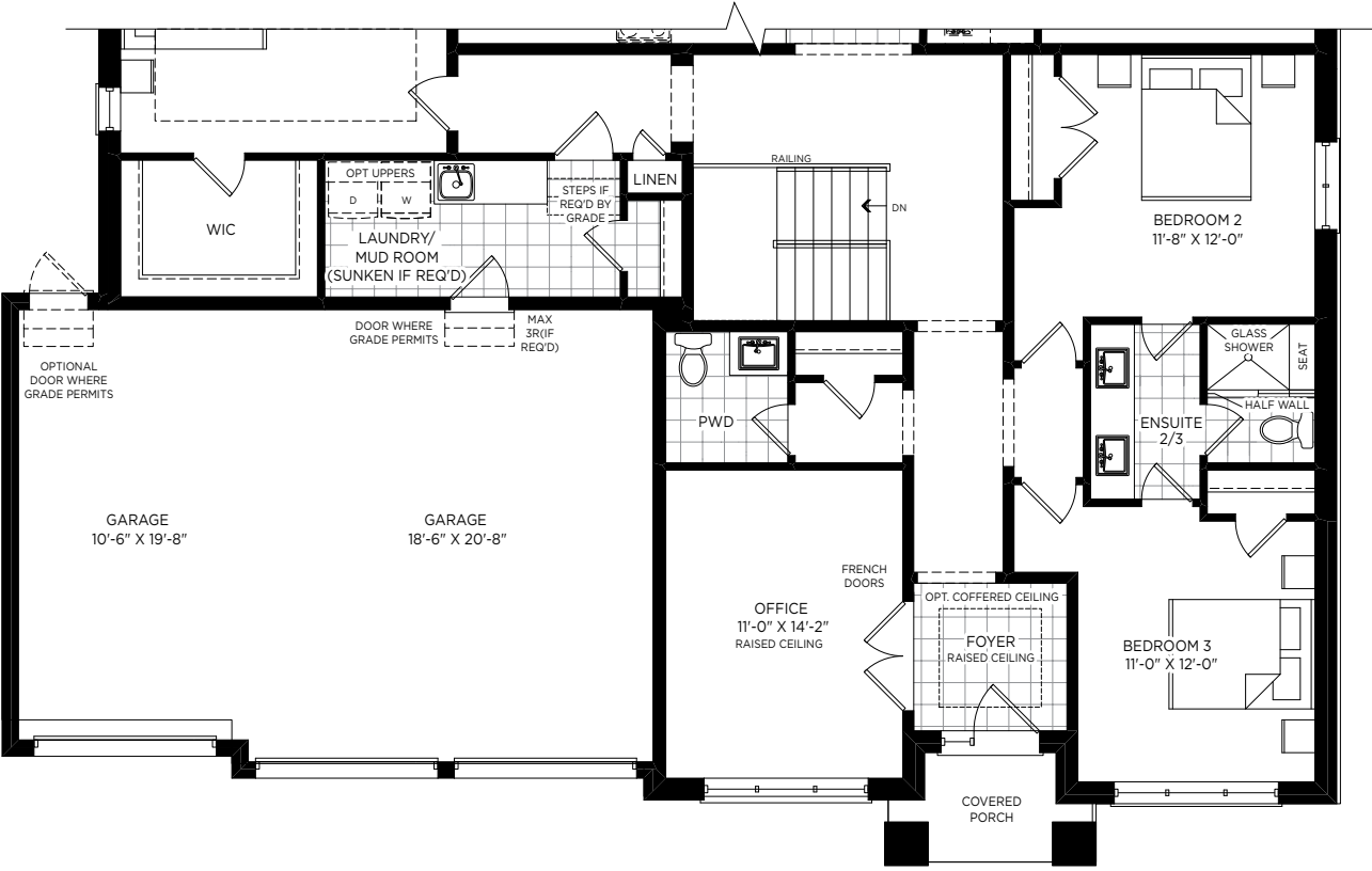
OPT. GROUND FLOOR WITH THIRD BEDROOM ELEVATION A
