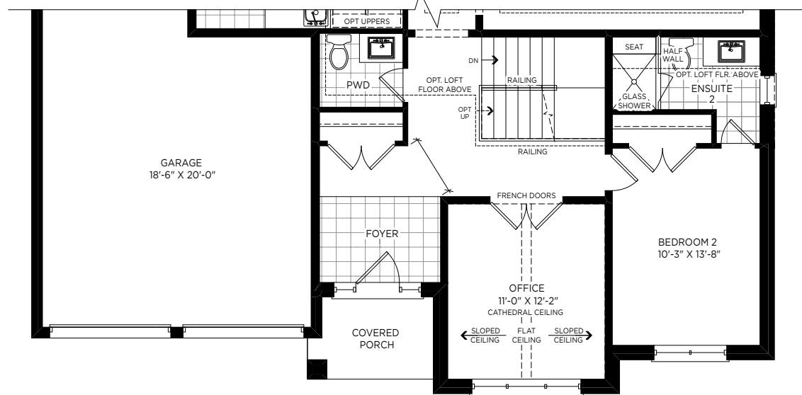
GROUND FLOOR ELEVATION B
