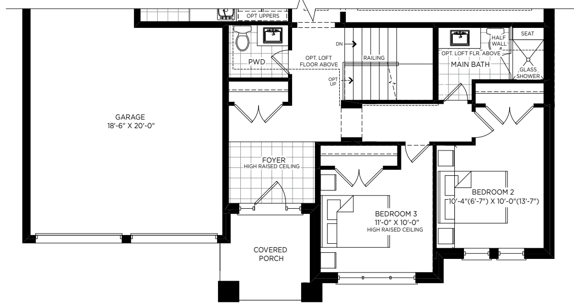
OPT. GROUND FLOOR WITH THIRD BEDROOM ELEVATION A
