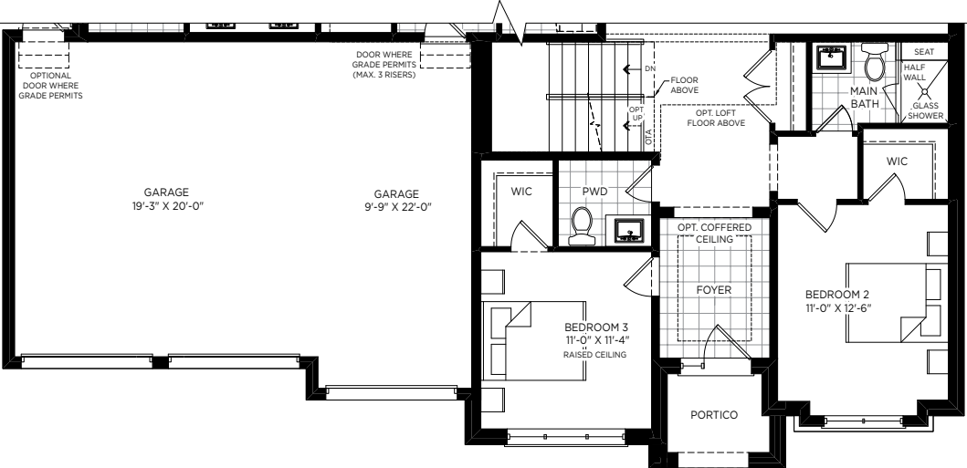
OPT. GROUND FLOOR WITH THIRD BEDROOM ELEVATION B
