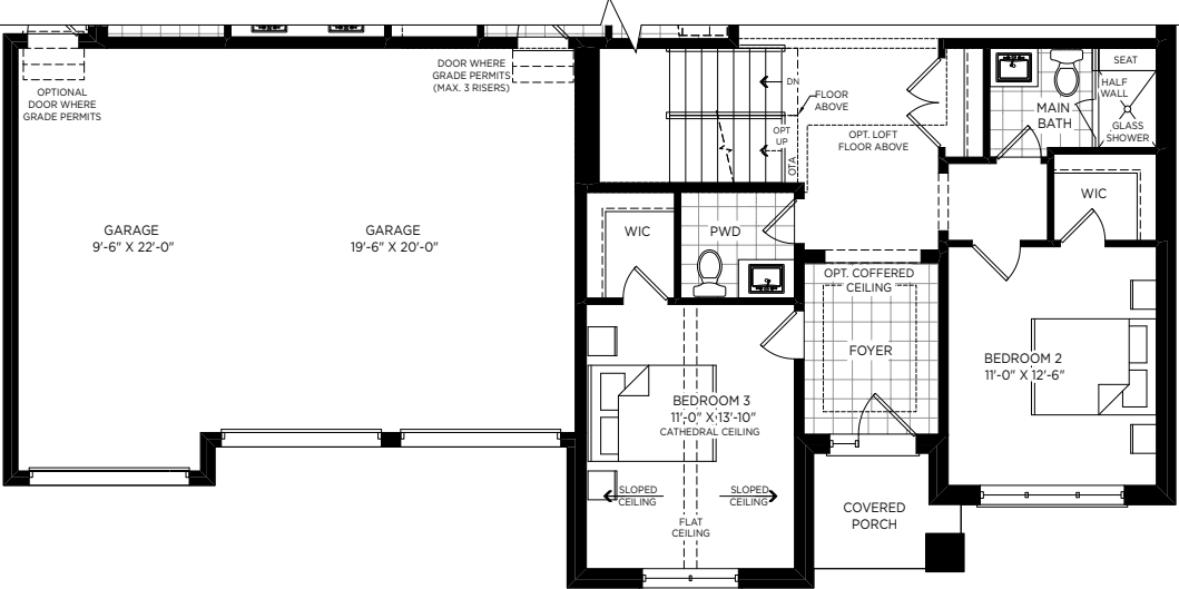
OPT. GROUND FLOOR WITH THIRD BEDROOM ELEVATION A
