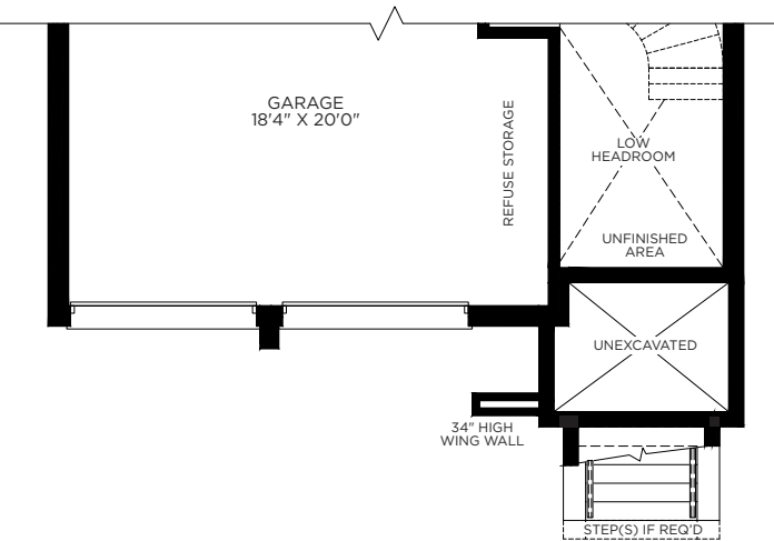
PARTIAL GROUND FLOOR PLAN ELEVATION B
