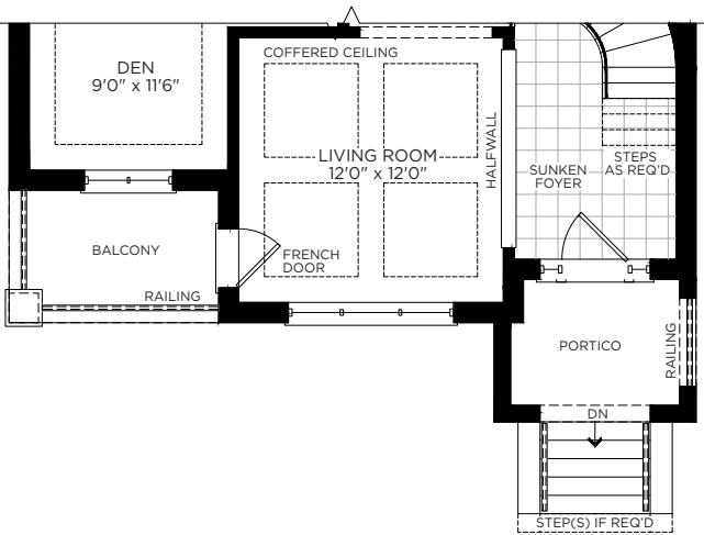
PARTIAL MAIN FLOOR PLAN ELEVATION B
