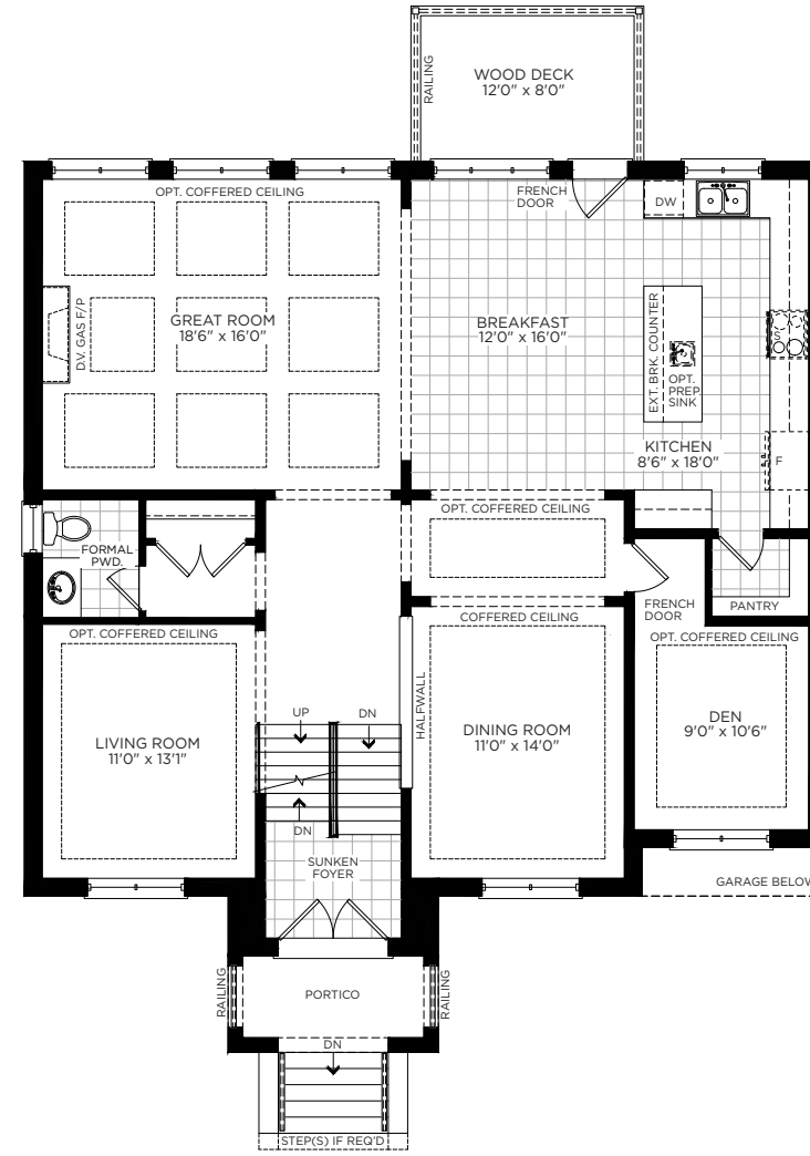
MAIN FLOOR PLAN ELEVATION B, LOT 16
