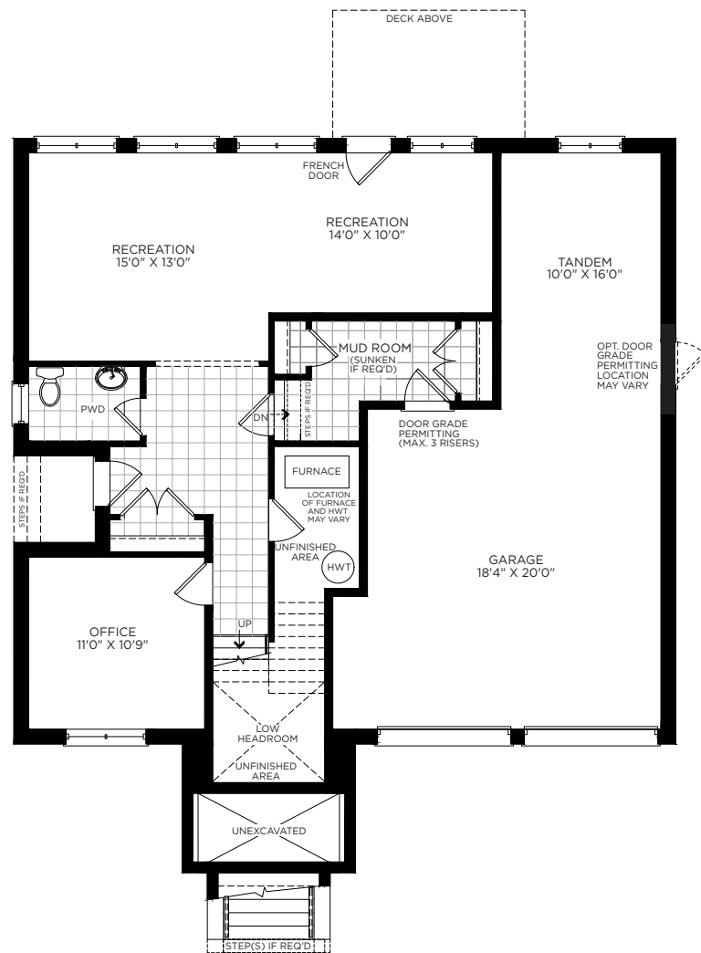
GROUND FLOOR PLAN ELEVATION B, LOT 16
