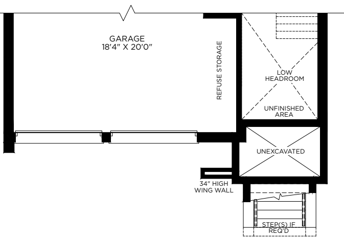
PARTIAL GROUND FLOOR PLAN ELEVATION B
